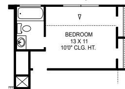
OPTIONAL BEDROOM 6 OR 7 W/ FULL BATH IN LIEU OF FLEX ROOM
